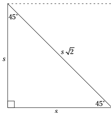
Figure 5-7: A 45-45-90 triangle is half of a square.
