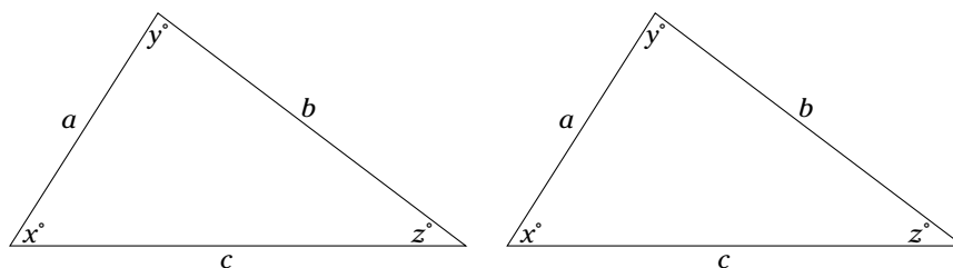
Figure 5-10: A pair of congruent triangles.
