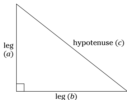
Figure 5-5: The Pythagorean theorem states that a^2 + b^2 = c^2 for any right triangle.
