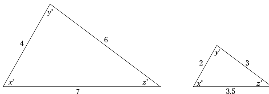
Figure 5-11: A pair of similar triangles.
