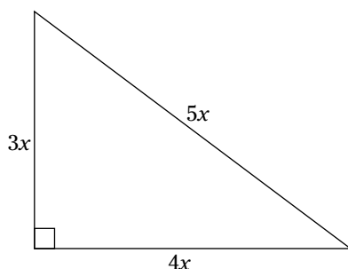
Figure 5-6: A 3-4-5 right triangle.
