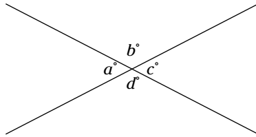
Figure 5-1: Vertical angles are equal.
