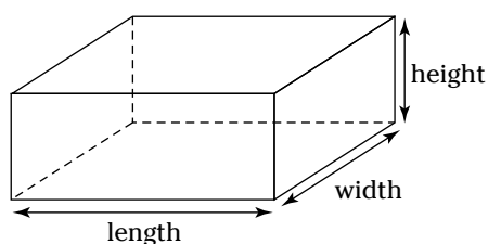
Figure 5-17: A rectangular solid.
